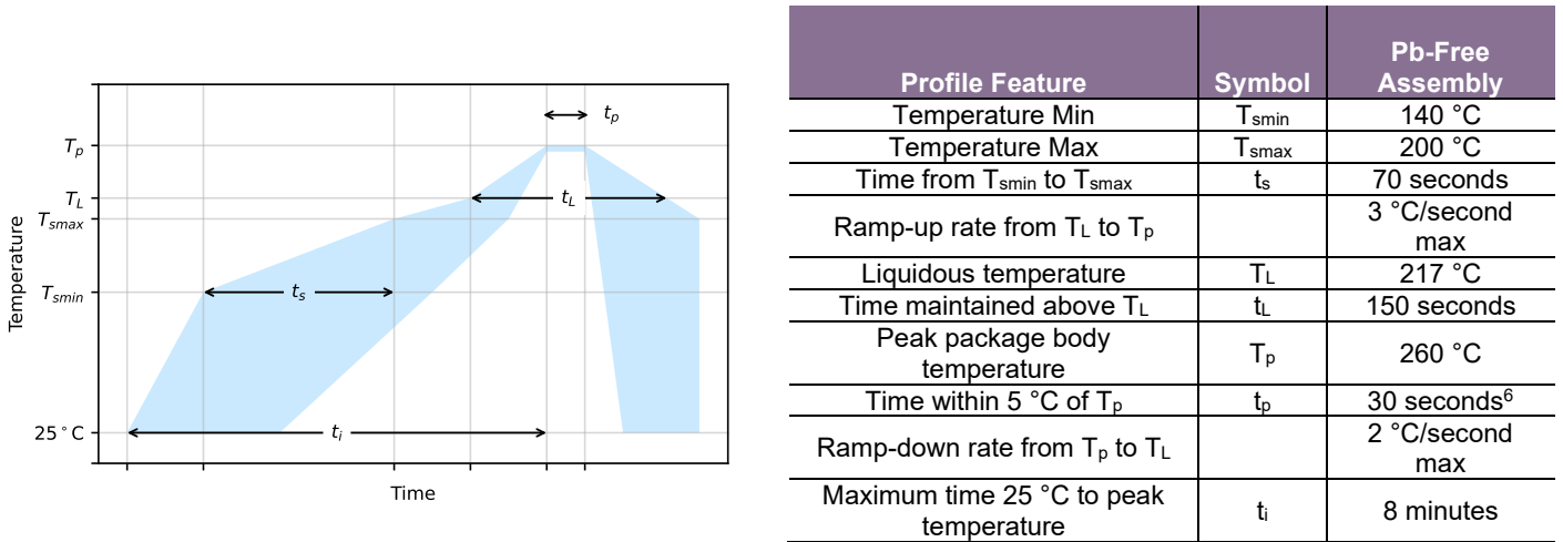
Figure 8.5: Reflow profile
