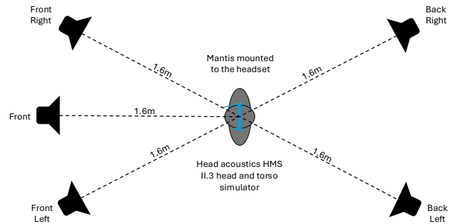
Figure 13: 360 Distractor Testing Setup
