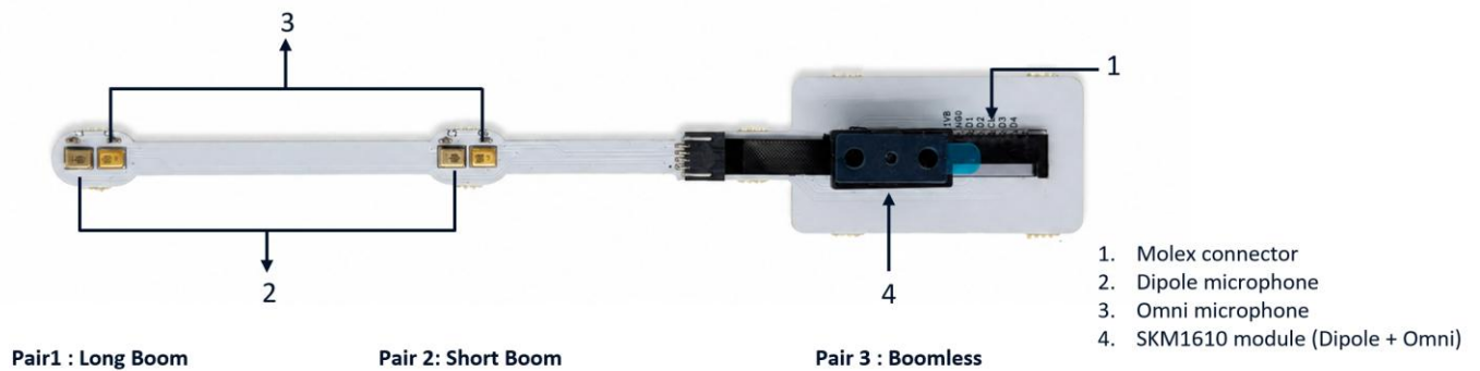
Figure 2: Mantis Board Microphone Pairs
