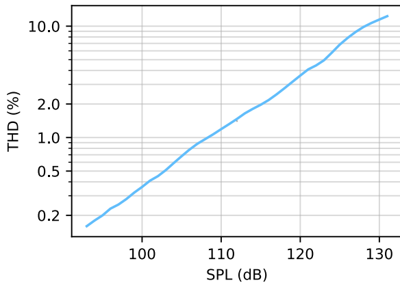
Figure 8.7: 1 kHz THD vs SPL
