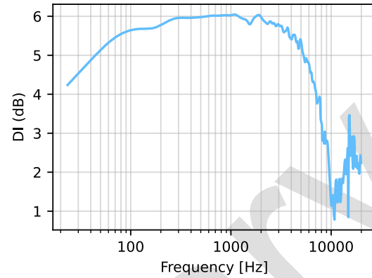
Figure 8.2: Directionality index vs frequency
