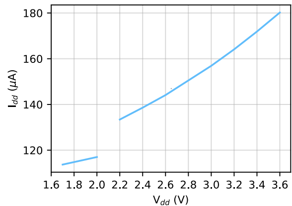
Figure 8.6: Supply current vs input voltage
