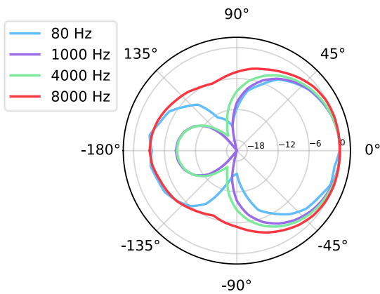
Figure 8.1: Polar pattern
