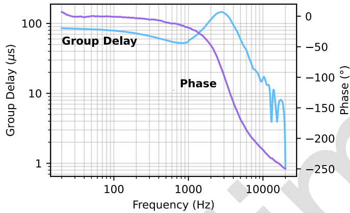
Figure 8.9: Phase and group delay
