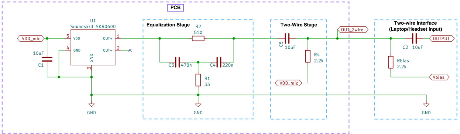
Figure 4.1: SKR0600 electrical two-stage circuit
