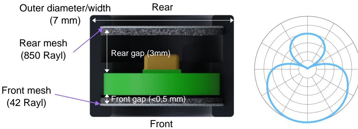
Figure 5.2: Cross section and polar pattern orientation
