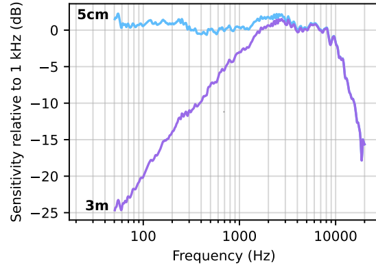
Figure 3.2: Sensitivity vs frequency
