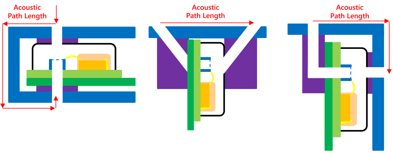
Figure 5: Acoustic path (red) for the thru-hole (left), V (middle), and L (right) configurations
