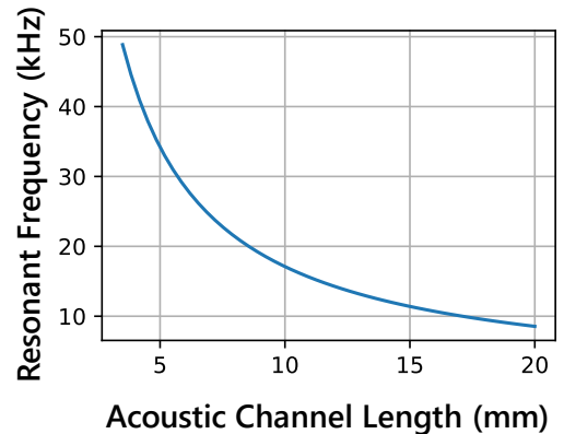
Figure 8: Resonant frequency vs. acoustic channel length
